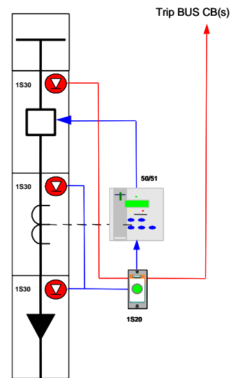
Figure 6: Two point sensors in zone 1 - Cable box and CT chamber One point sensor in zone 2 for CB chamber
