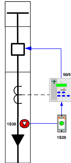
Figure 4: Single point sensor - Cable box
