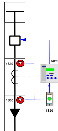
Figure 5: Two point sensors - Cable box and CT chamber
