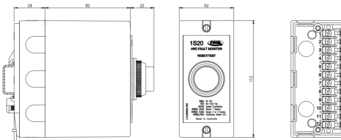
Figure 19: DIN rail mounting detail
