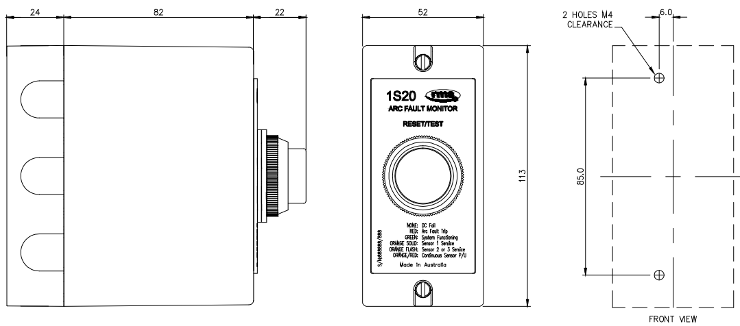
Figure 18: Surface mounting detail
