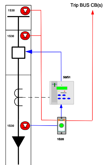
Figure 7: One arc sensor - Cable box / CT chamber Independent trip to CB Two arc sensors - CB chamber & BUS chamber Independent trip to BUS breaker (BUS overcurrent check stage not shown)
